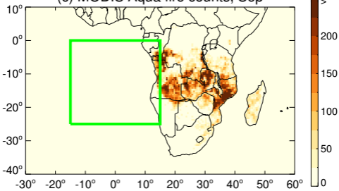
(c) MODIS Aqua fire counts, Sep
