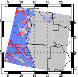
(e) Neighbour difference mask
