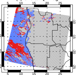
(b) Overall QA flag
