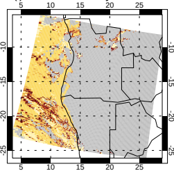
(i) AOD uncertainty estimate
