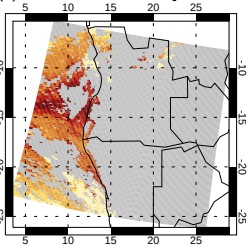
(h) Above-cloud AOD, QA filtered
