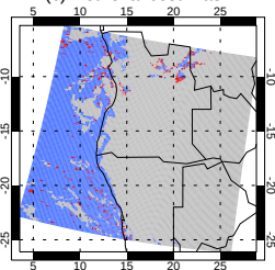
(c) Retrieval cost mask
