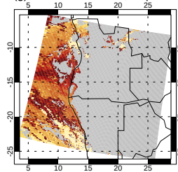
(g) Above-cloud AOD, all points
