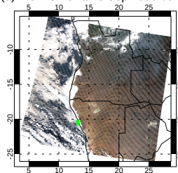
(a) MODIS Terra 13 Sep 2000 09:25
