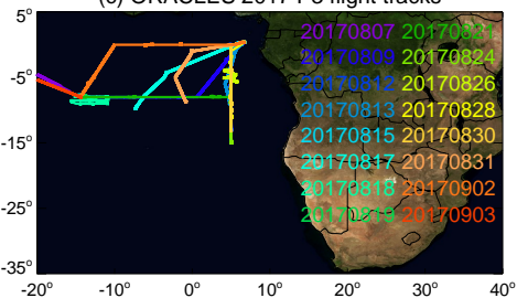
(c) ORACLES 2017 P3 flight tracks
