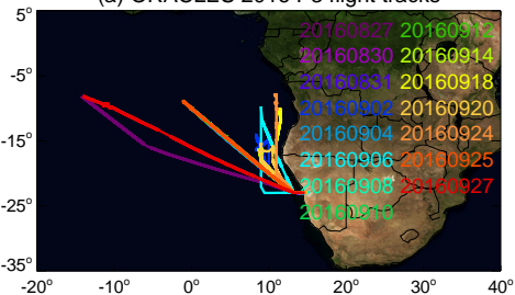
(a) ORACLES 2016 P3 flight tracks
