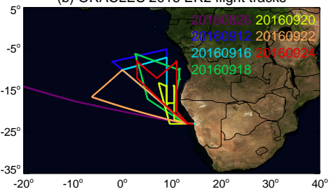
(b) ORACLES 2016 ER2 flight tracks
