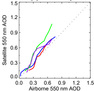
(b) MODIS Aqua
