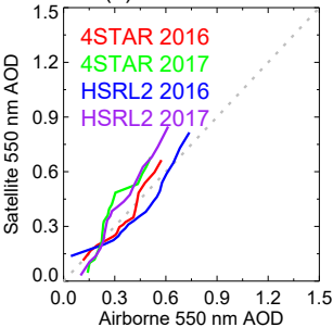
(a) MODIS Terra
