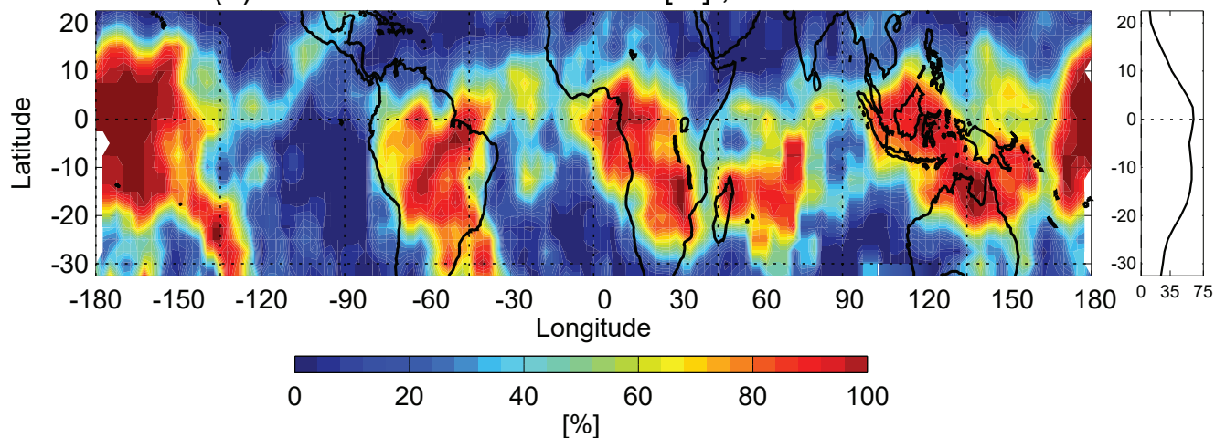
(b) TANSO-FTS cirrus fraction [%] , 25–31 Jan 2010
