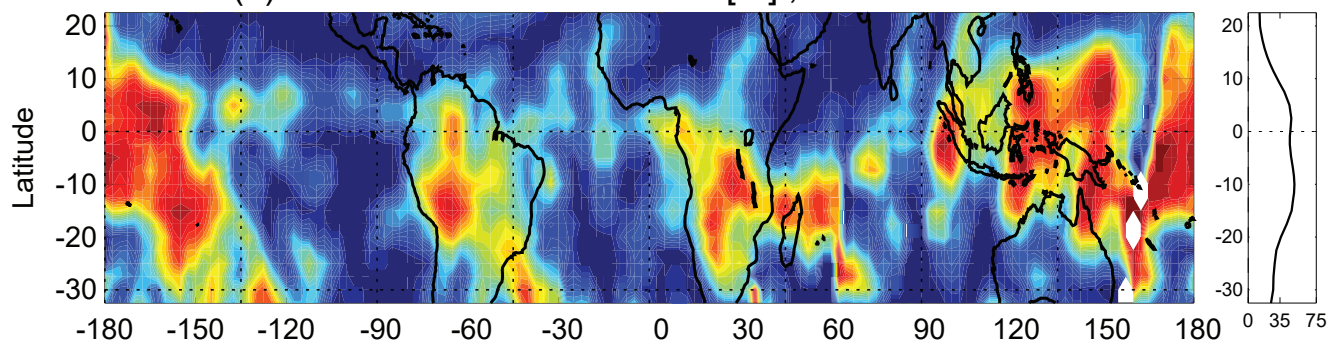
(b) TANSO-FTS cirrus fraction [%] , 25–31 Jan 2010
