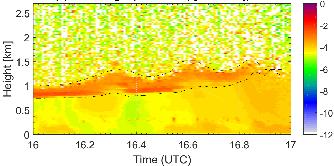
(b) HSRL circular depol ratio
