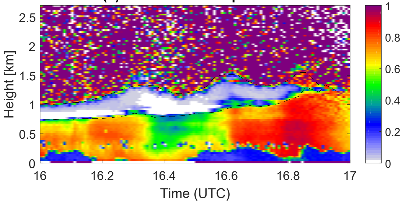
(b) HSRL circular depol ratio
