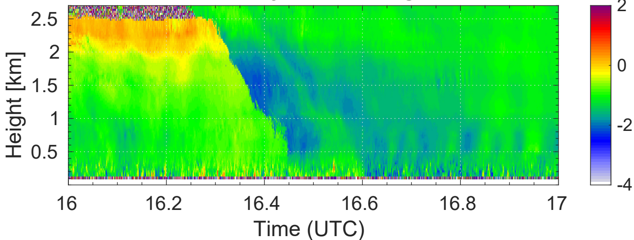
(c) Spectrum width [ \text{m s}^{-1} ]
