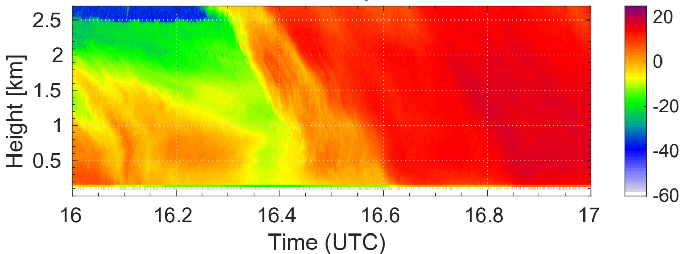
(b) Doppler velocity [ \text{m s}^{-1} ] (neg. = down)
