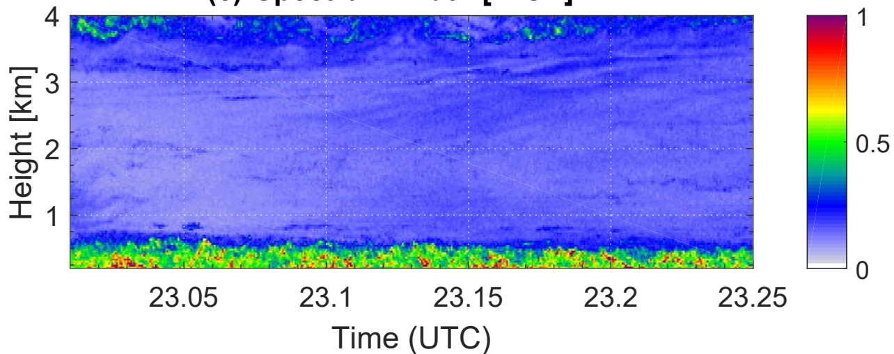
(c) Spectrum width [m s -1 ]
