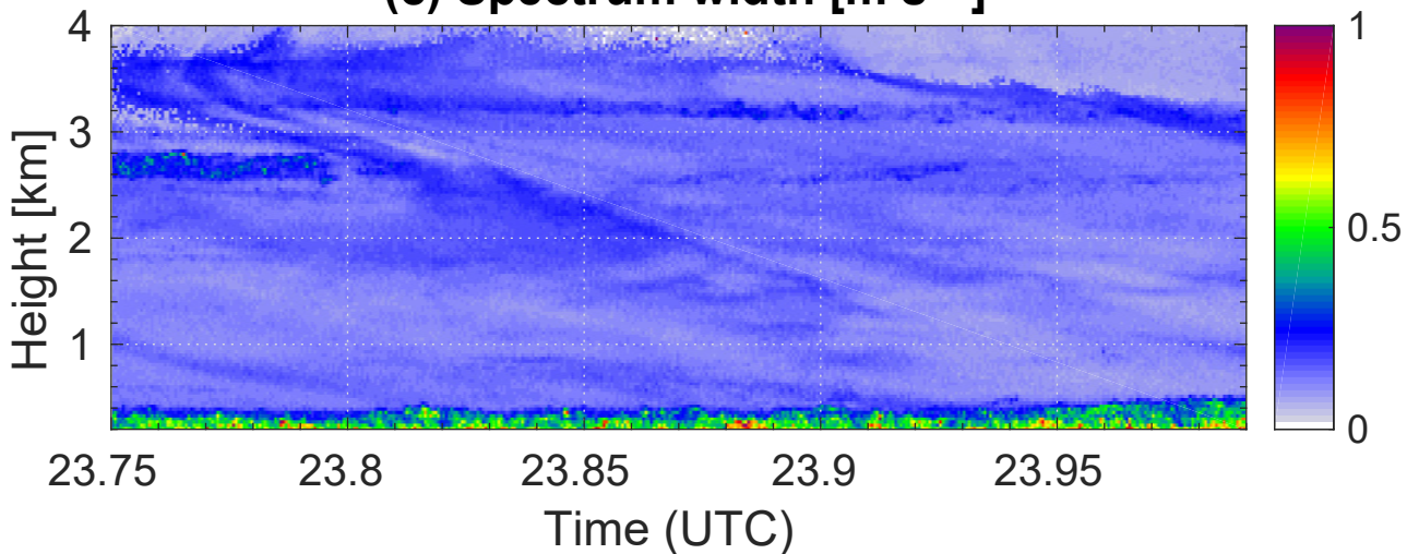
(c) Spectrum width [ \text{m s}^{-1} ]
