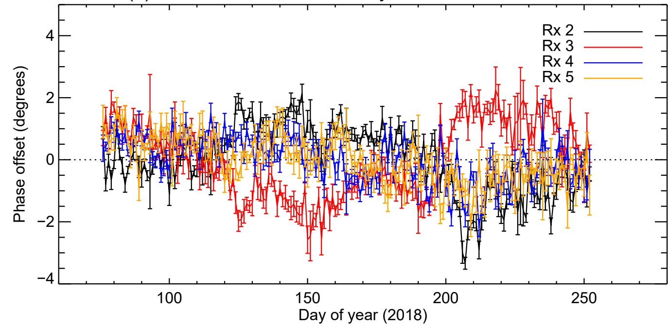
(b) Phase correction variability for BP meteor receivers
