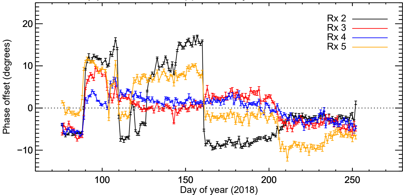
(b) Phase correction variability for BP meteor receivers
