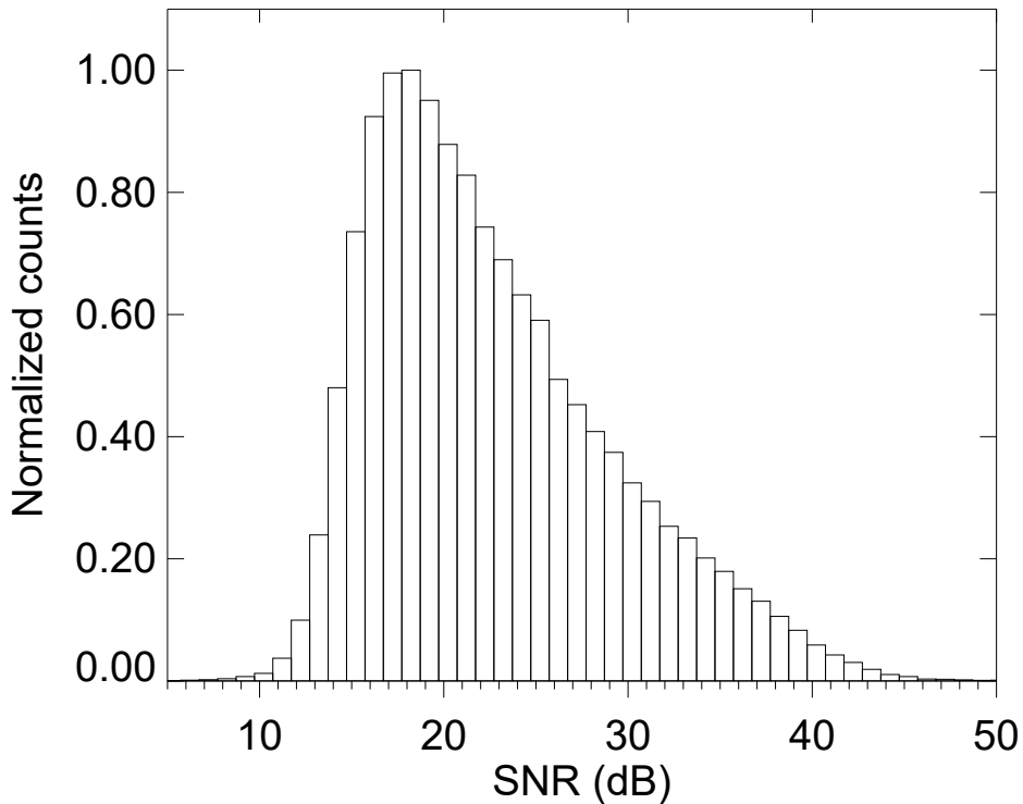
SNR distribution
