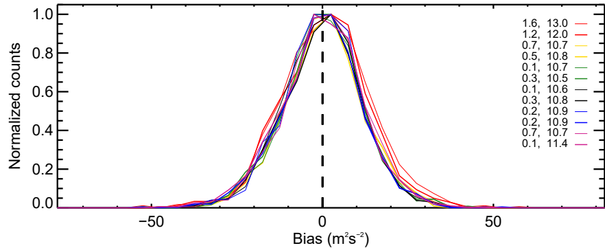
Simulated covariance, \langle v'w' \rangle
