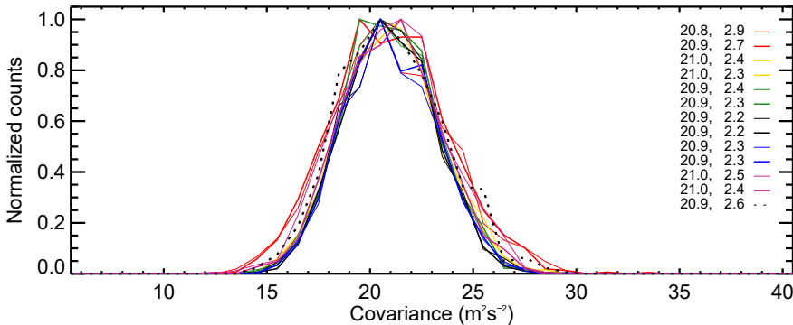
Simulated covariance, \langle u'w' \rangle
