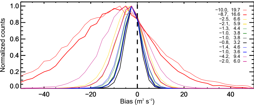
Bias in covariance, \langle u'w' \rangle
