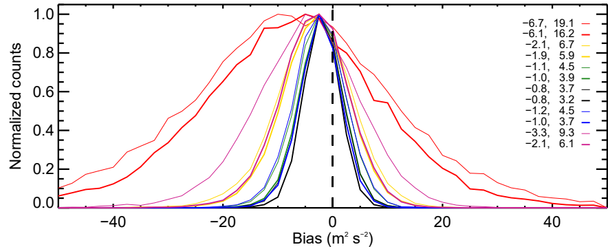
Bias in covariance, \langle v'w' \rangle
