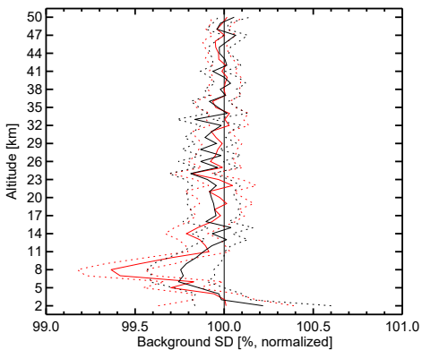
(a) ATMS
