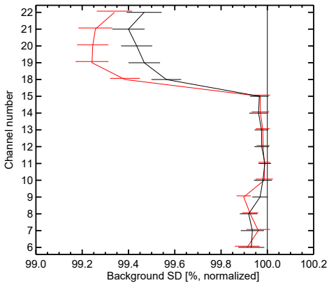
(a) ATMS
