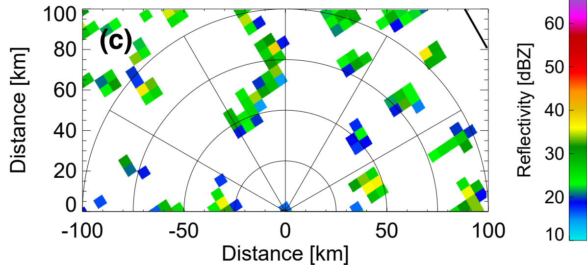
GPM-DPR Ku-NS 04/03/2018 09:15:10 / 1 km
