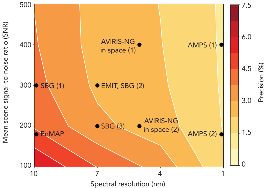
Precision of methane retrievals from imaging spectrometers
