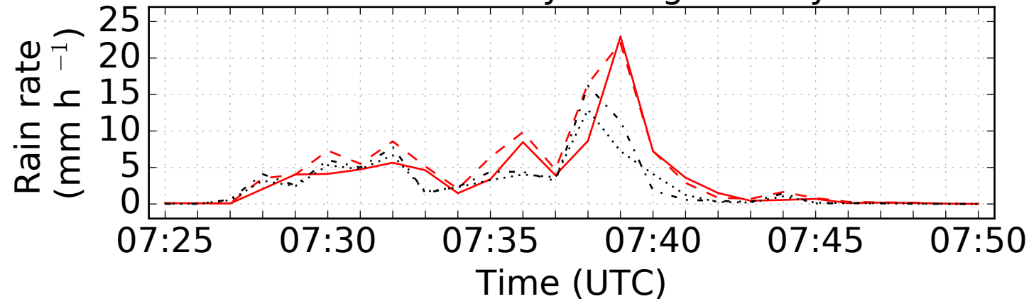
Rain rate observed by four disdrometers at Chilbolton Observatory during a heavy shower.
