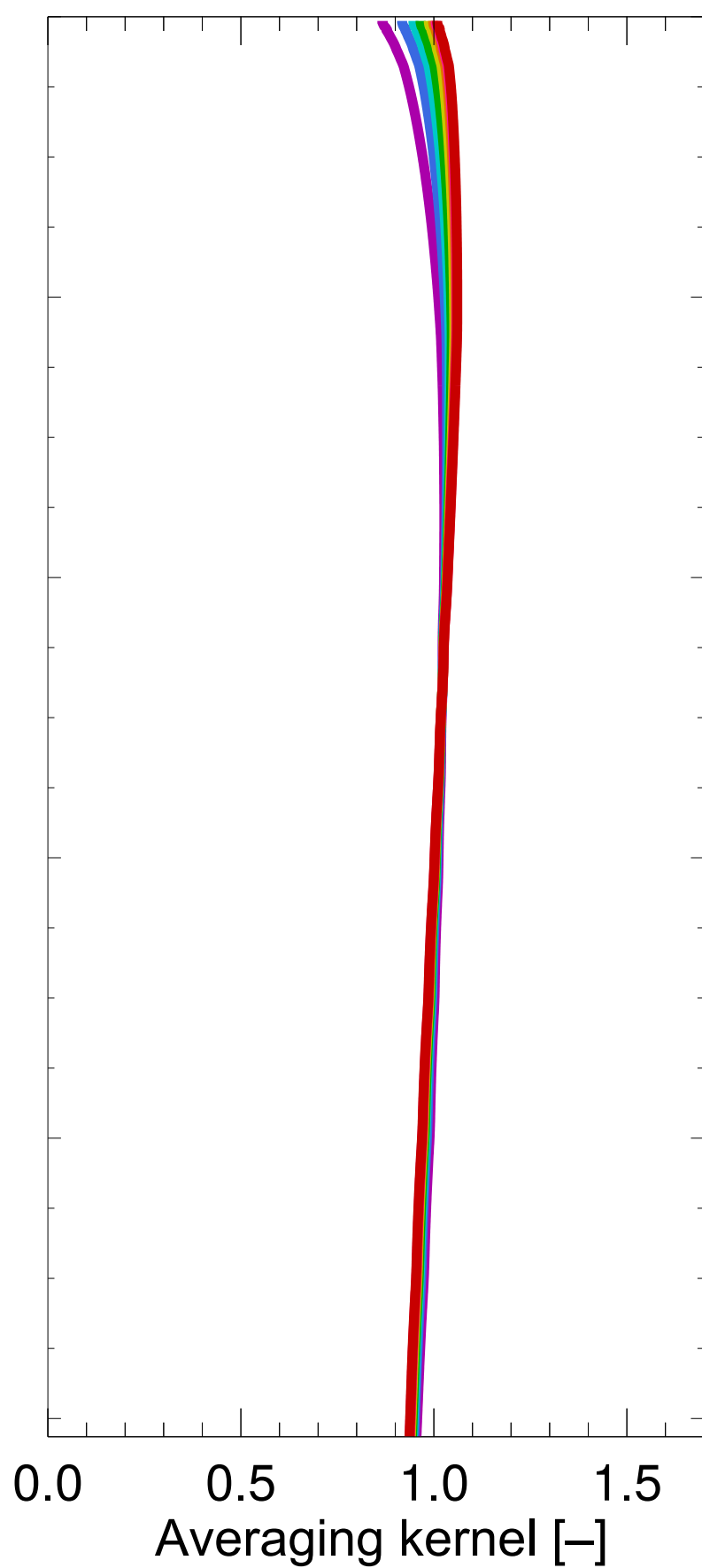
TROPOMI/WFMD CO
