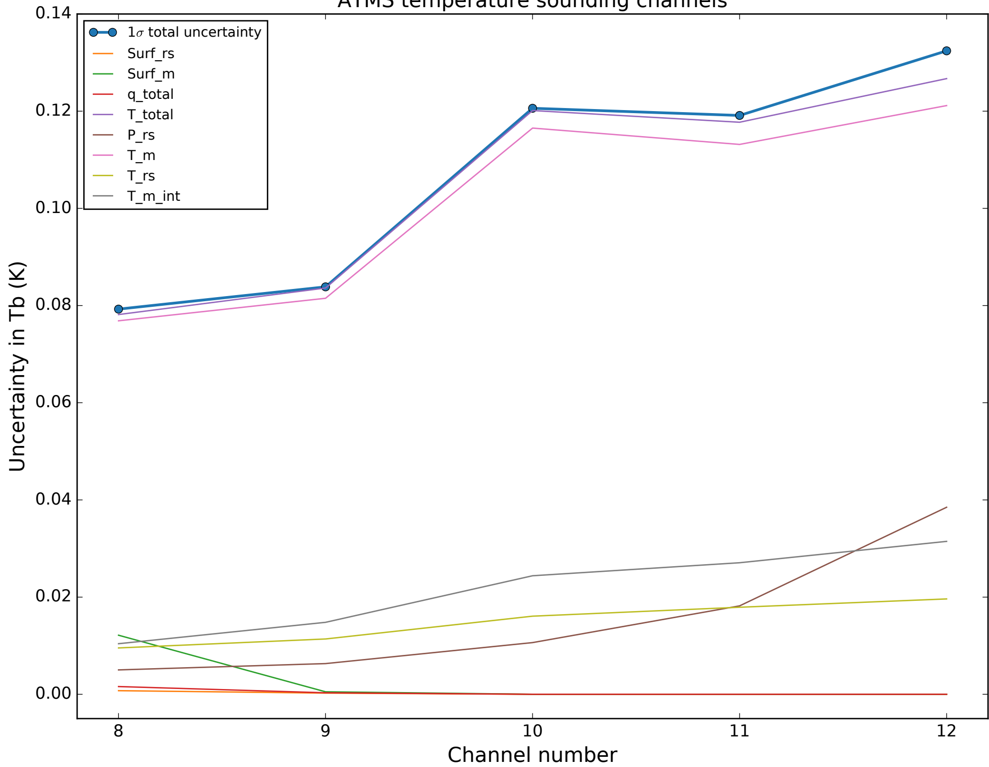
ATMS temperature sounding channels
