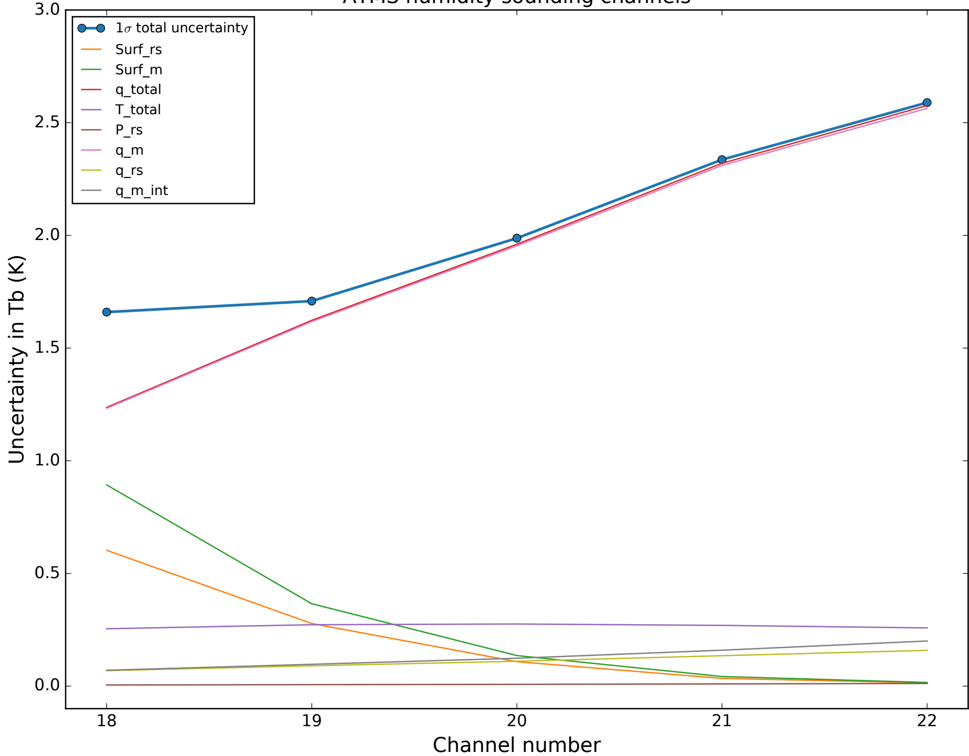
ATMS humidity sounding channels
