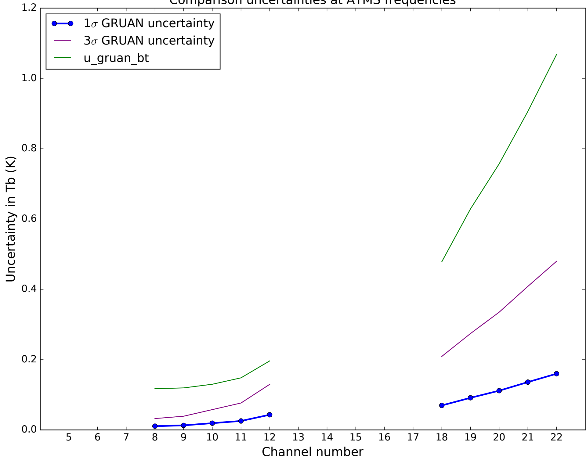
Comparison uncertainties at ATMS frequencies
