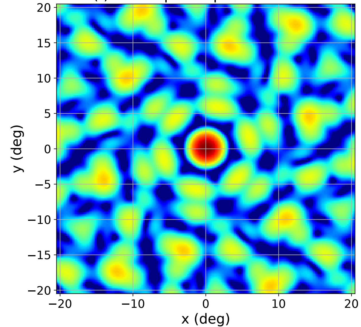
(f) MIMO: point spread function
