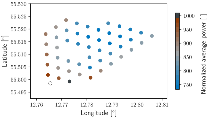
(a) Lillgrund layout; wind turbines are filled markers; met mast is open marker
