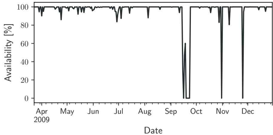
(b) Daily data availability from met mast
