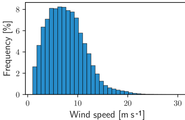
(a) Histogram of wind speed
