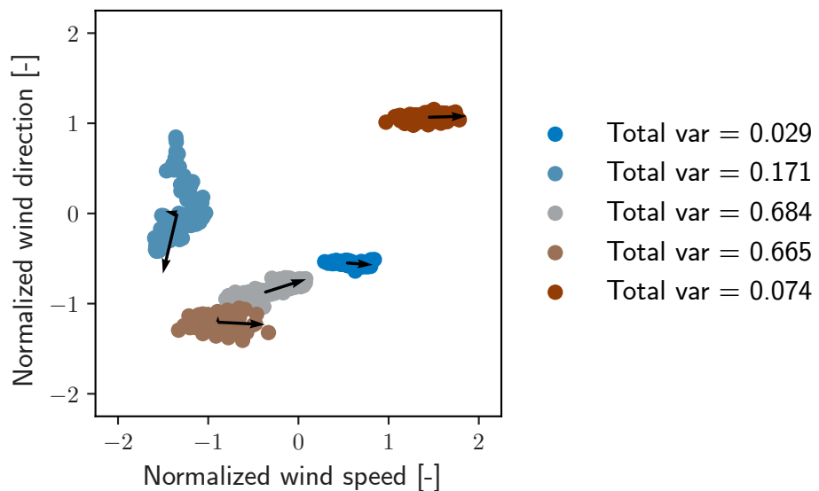
(b) Scatter of observations in selected time periods
