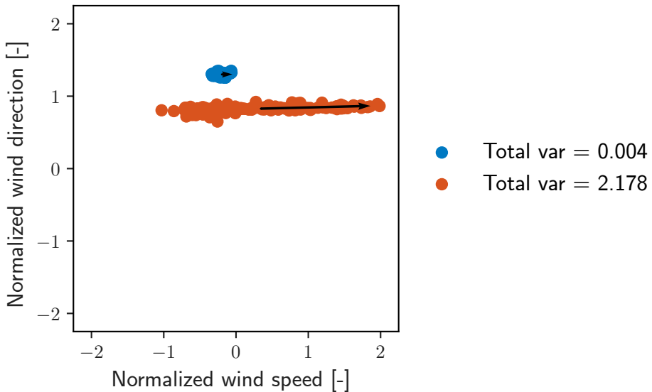
(a) Time periods exhibiting the lowest and highest values of total variation (blue and red, respectively)
