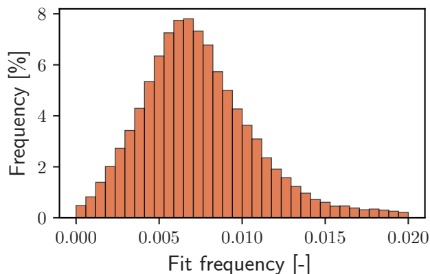
(d) Distribution of frequency, c_0 from eq. (8)
