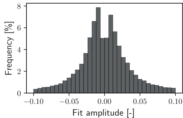
(e) Distribution of amplitude, c_0 from eq. (9)
