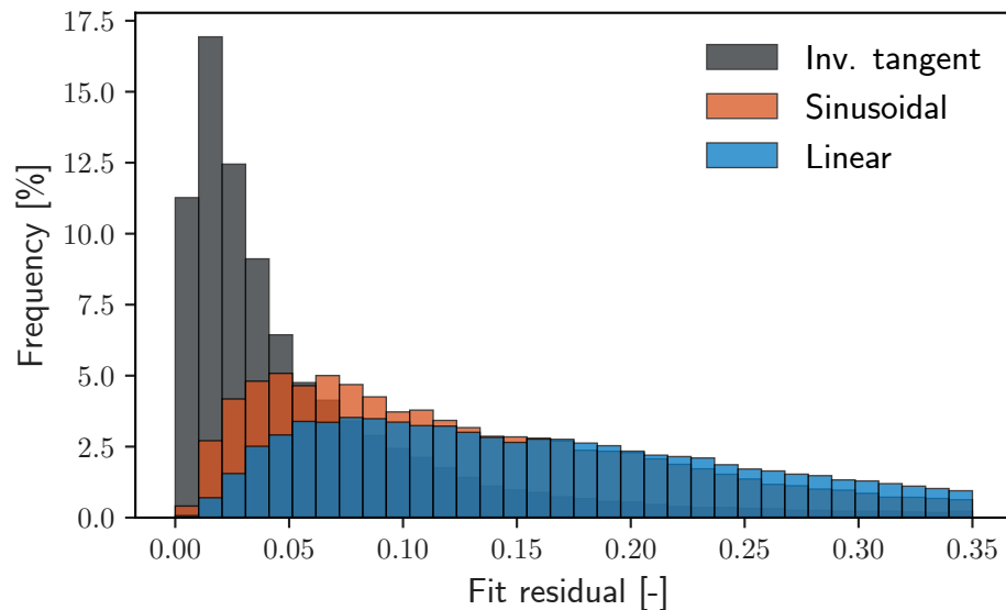
(b) Distribution of fit residuals
