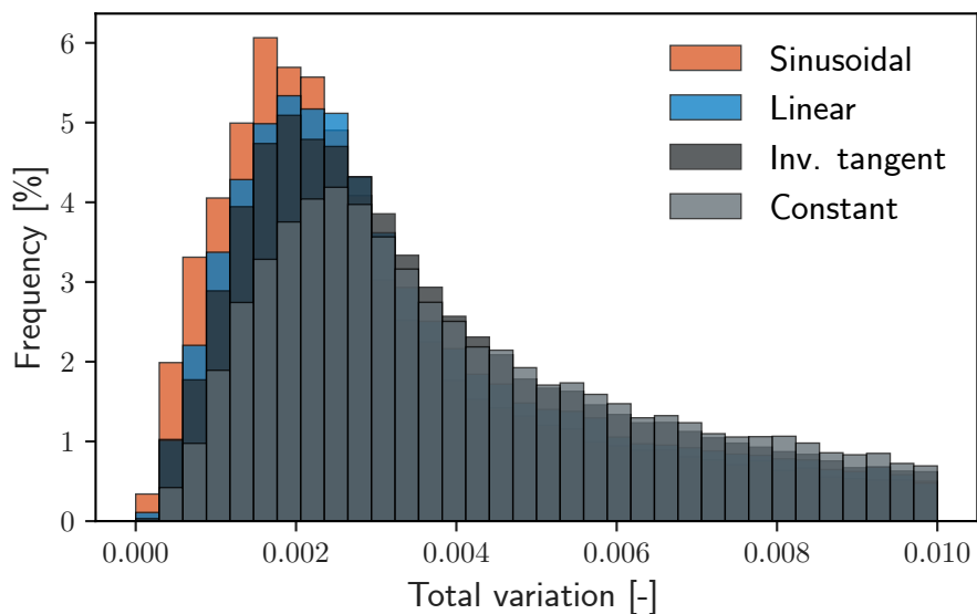
(a) Distributions of total variation for tested objective functions
