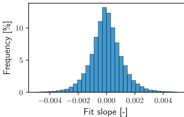
(c) Distribution of slope, c_0 from eq. (7)
