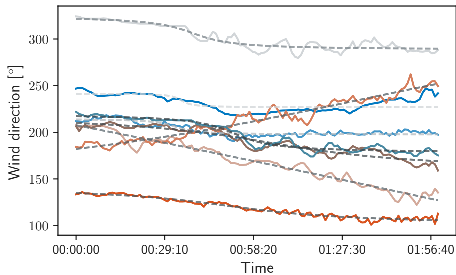
(c) Inverse tangent time series from met mast
