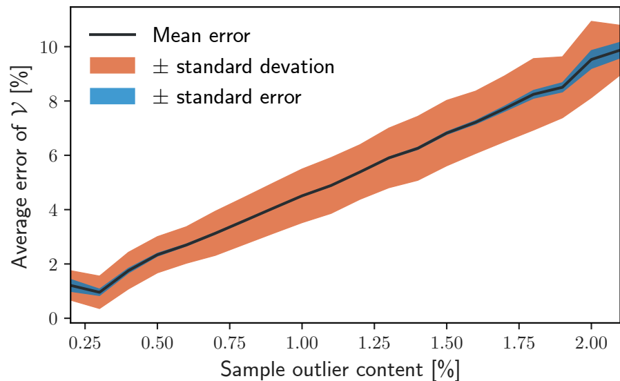
(d) Mean relative error due to the presence of outliers
