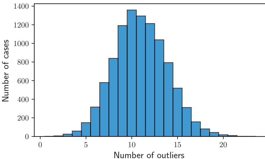
(c) Outlier detection in synthetic data
