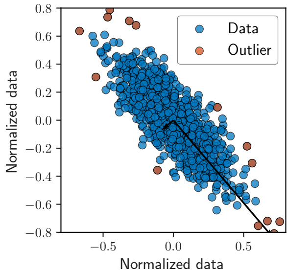
(a) Synthetic data and outliers
