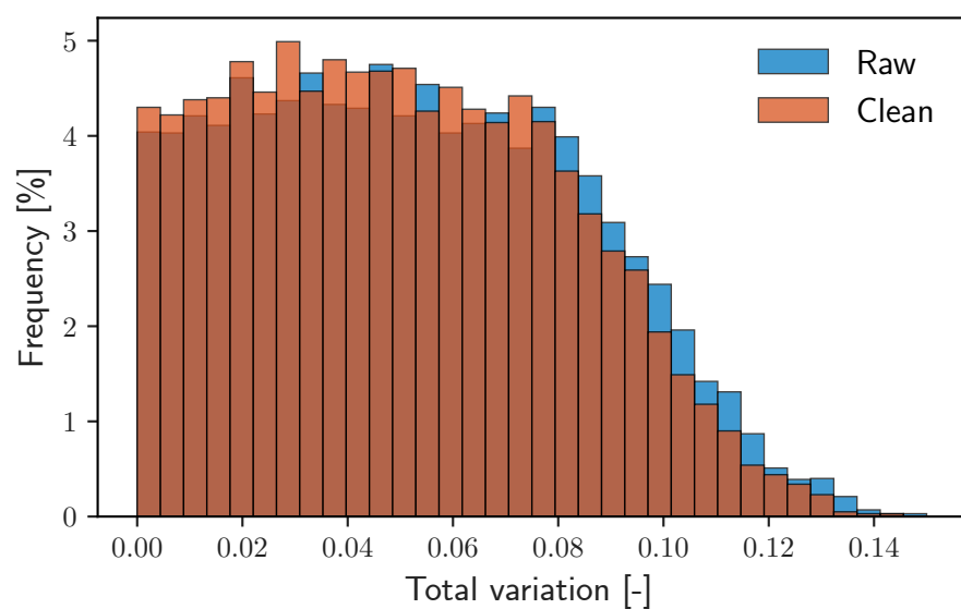
(b) Distribution of total variations with and without outliers
