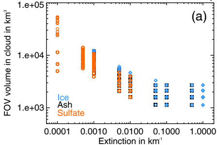
Cloud volume in FOV at detected cloud top
