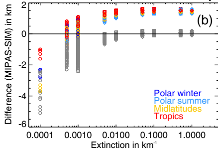
MIPAS cloud top altitude uncertainty
