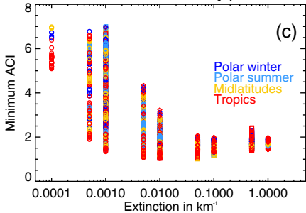
Minimum ACI of cloudy profiles
