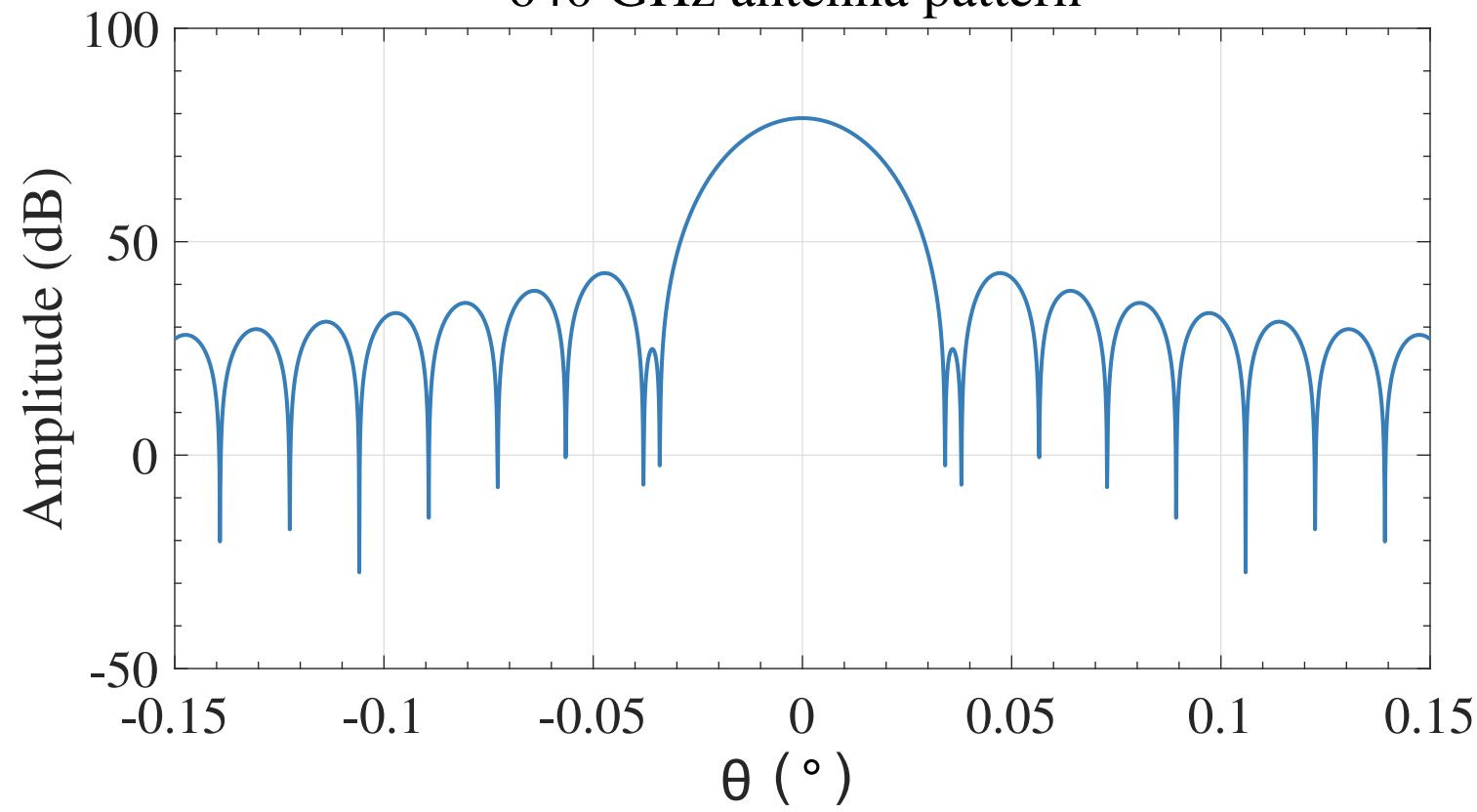
640 GHz antenna pattern
