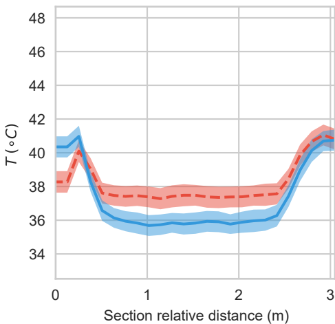
(c) Mean wind speed = 1.8 \text{ m s}^{-1}
