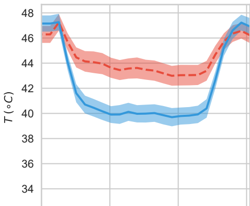
(a) Mean wind speed = 0.35 \text{ m s}^{-1}
