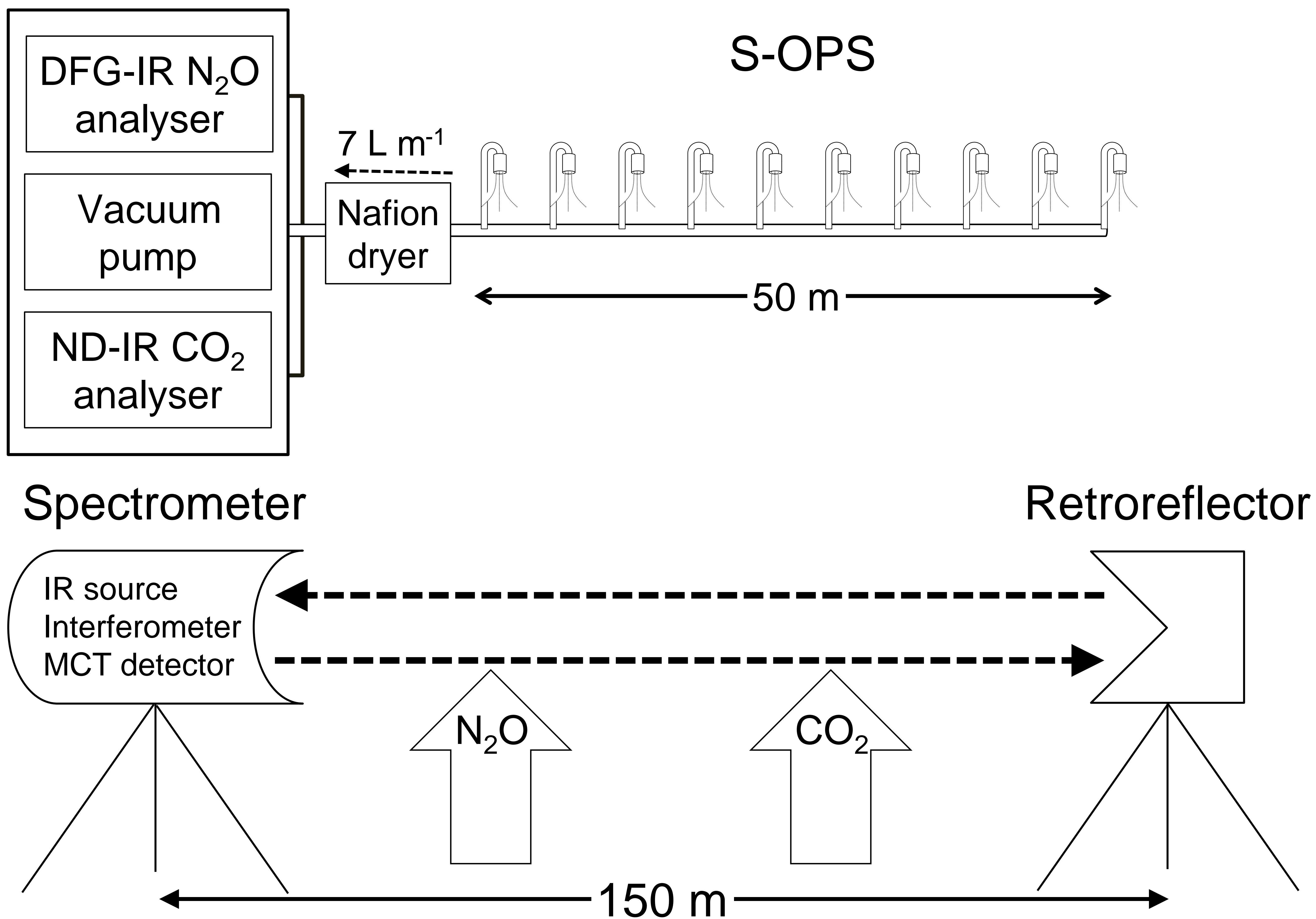
(b) A monostatic OP-FTIR
