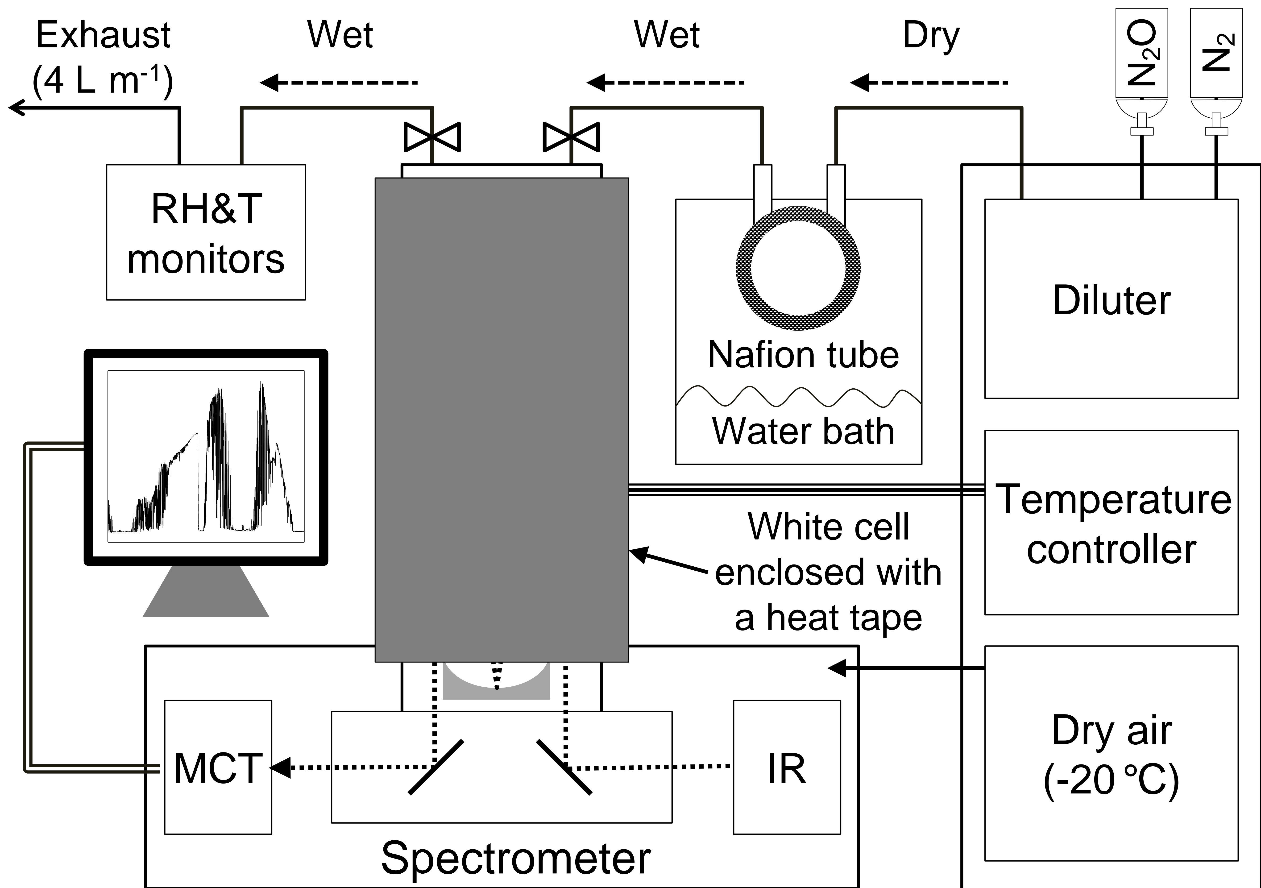
(a) A lab FTIR
