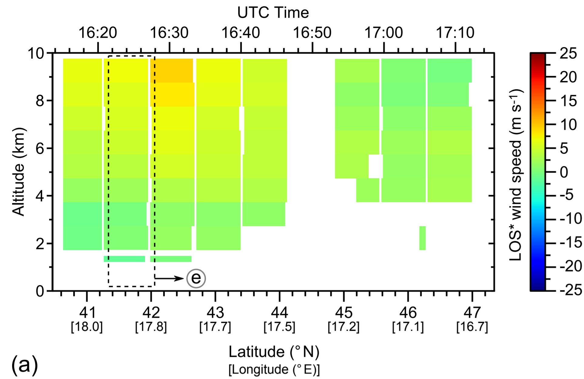
ECMWF LOS* winds
