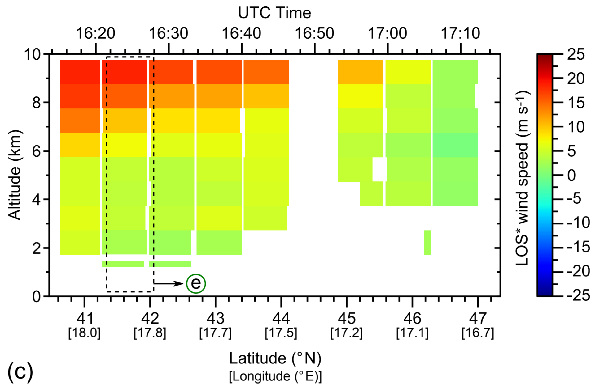
Aeolus L2B Rayleigh LOS* winds
