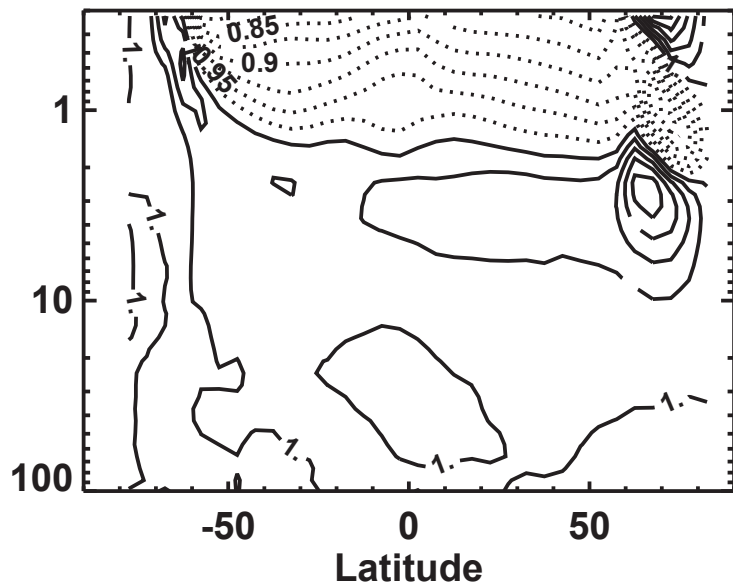
(c) Jun model ASC/DSC ratio
