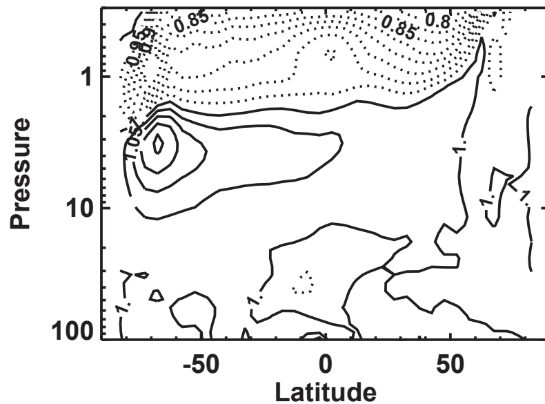
(b) Dec Aura MLS ASC/DSC ratio
