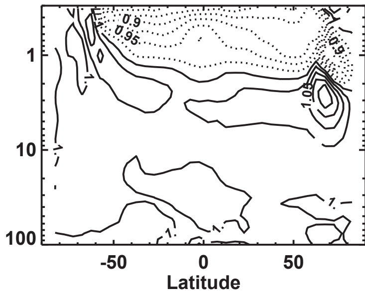
(a) Jun Aura MLS ASC/DSC ratio
