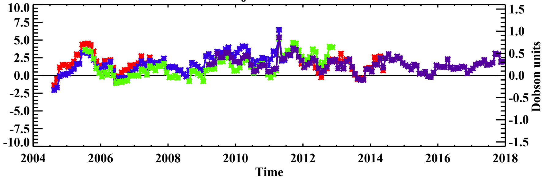
(b) SBUV adjusted to 13:30
