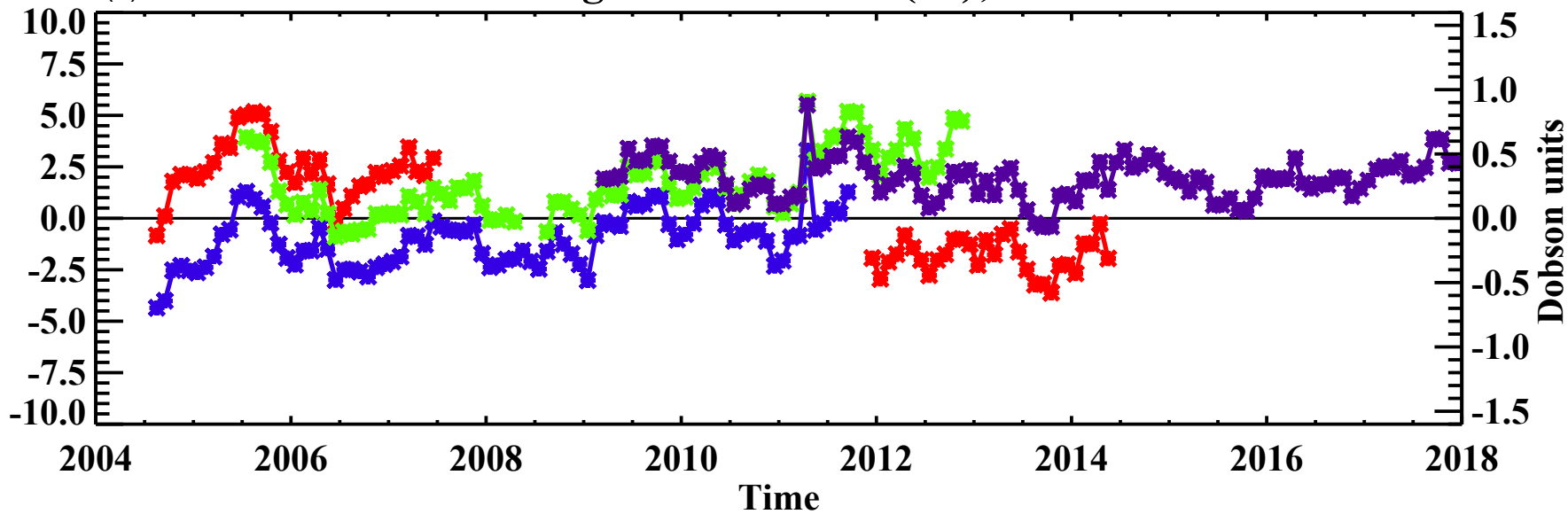
(a) 10–15° S zonal avg. SBUV - MLS (%); 6.39–4.03 hPa
