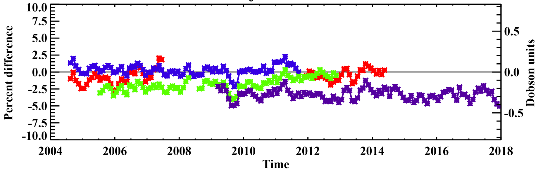
(b) SBUV adjusted to 13:30
