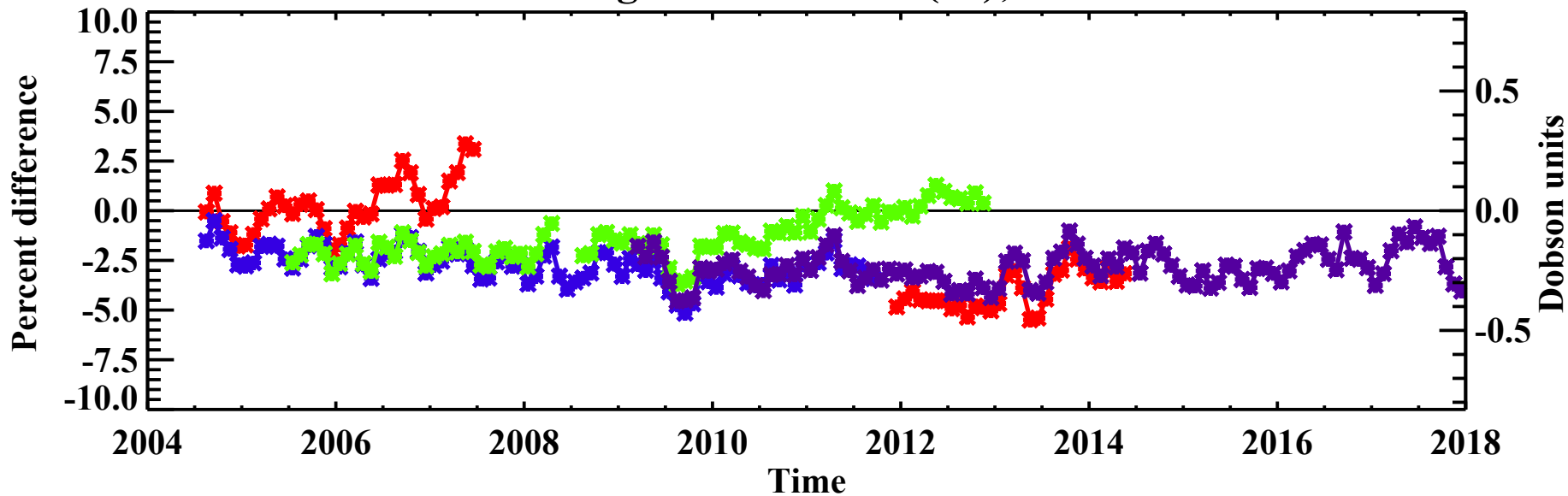
(a) 10–15° S zonal avg. SBUV - MLS (%); 4.03–2.55 hPa
