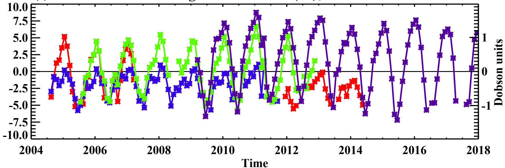
(a) 50–55° S zonal avg. SBUV - MLS (%); 10.13–6.39 hPa
