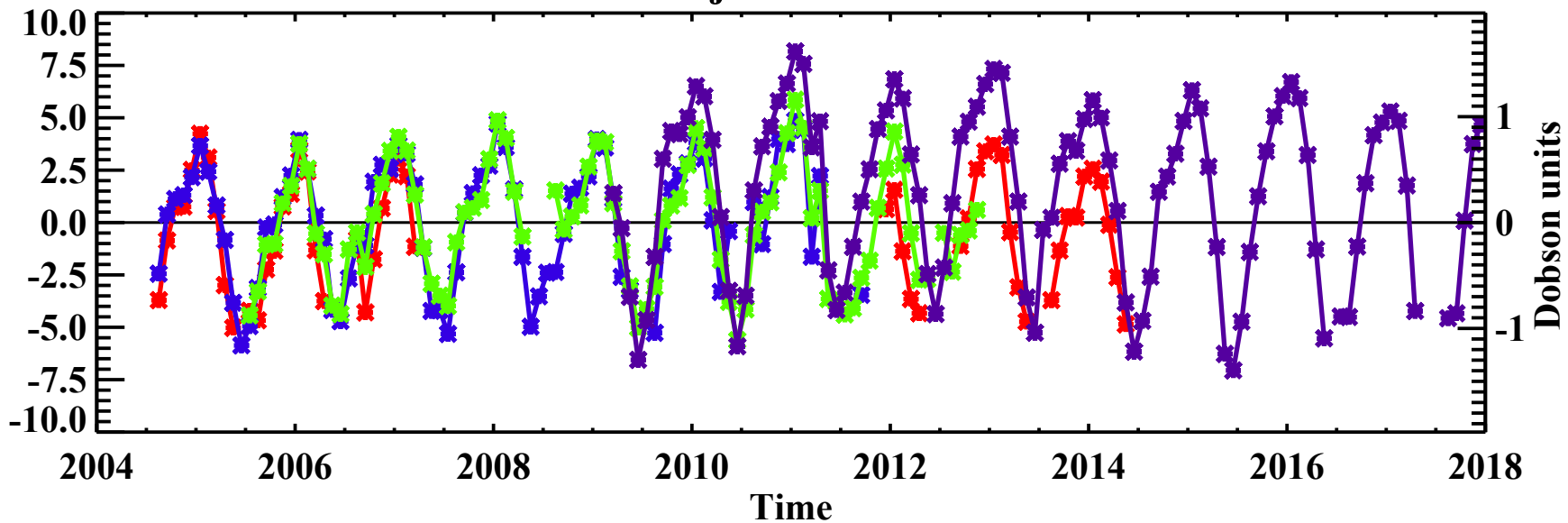
(b) SBUV adjusted to 13:30
