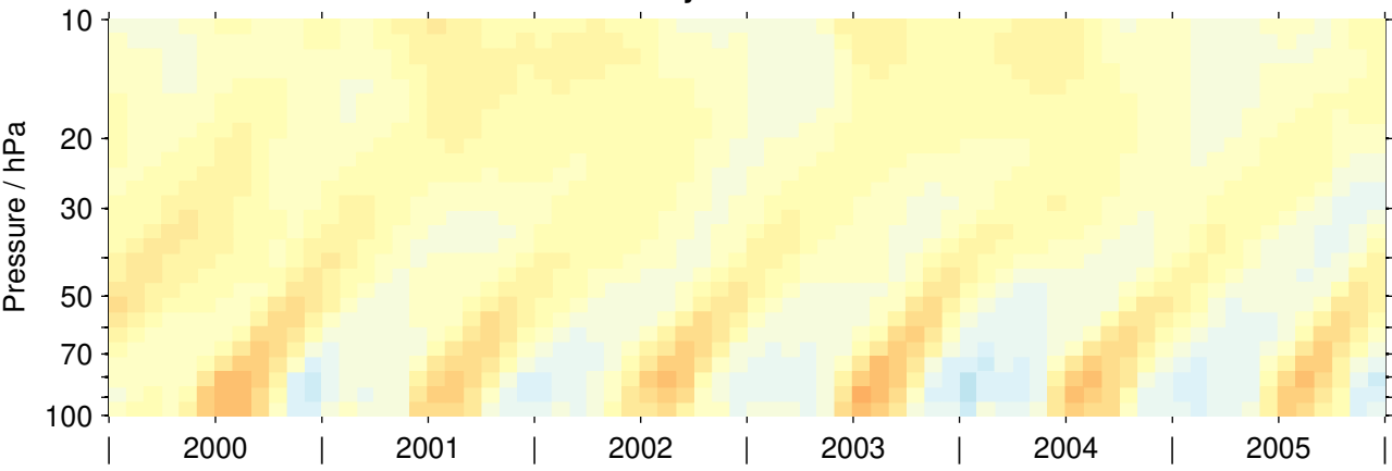
EMAC / January 2000–December 2005
