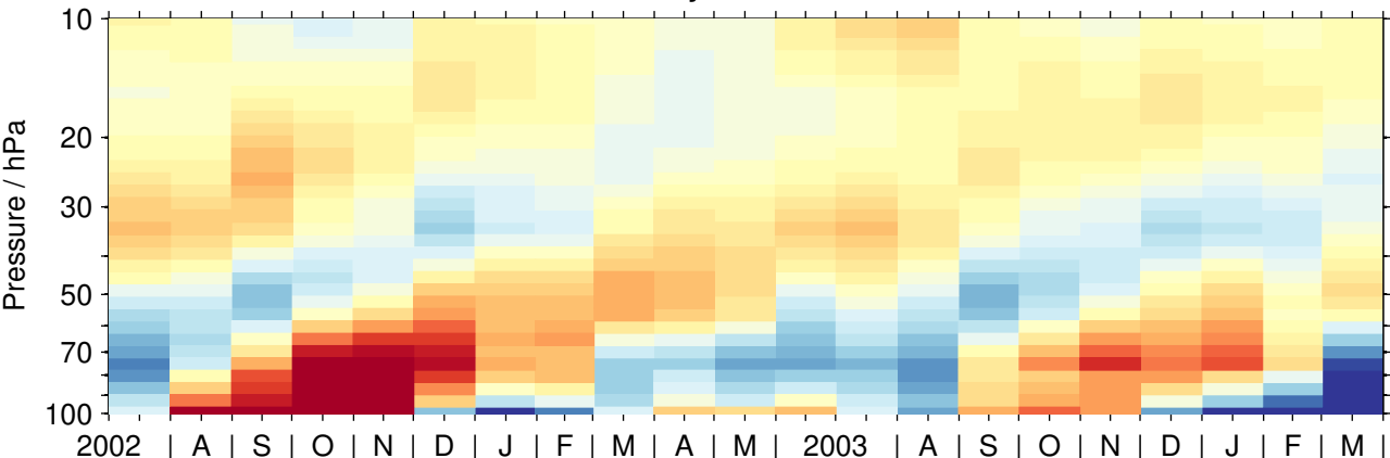
ACE-FTS / April 2004–November 2014
