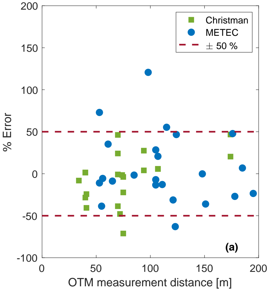
% Error vs. measurement distance
