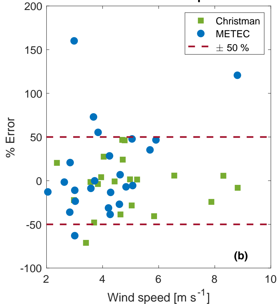
% Error vs. wind speed
