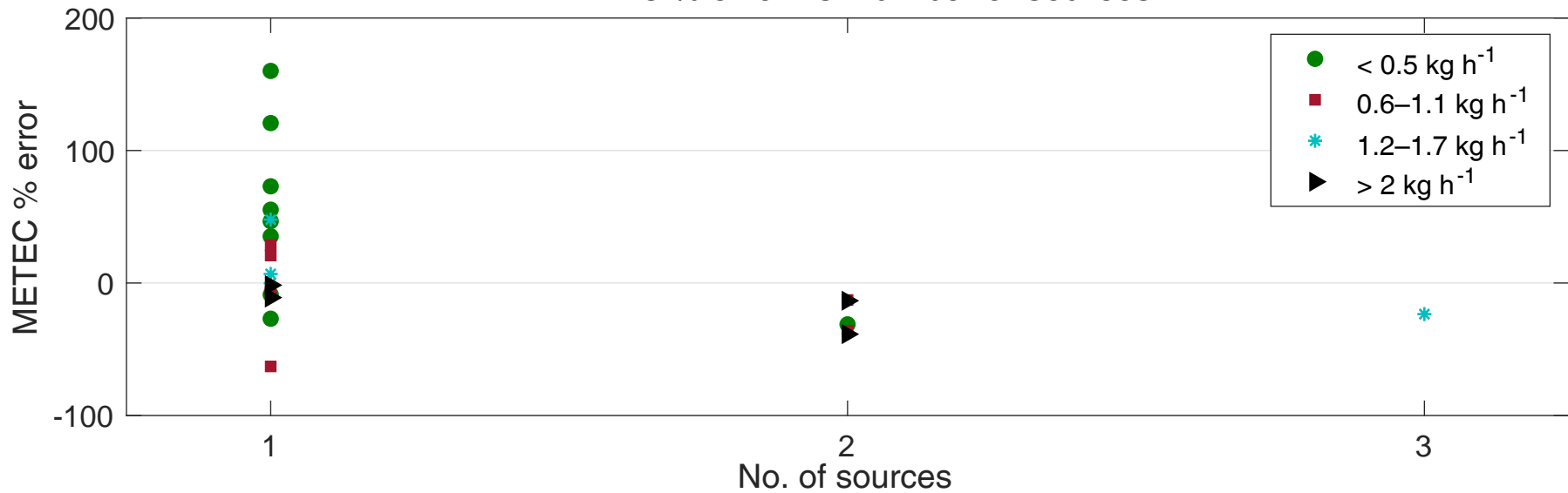
METEC % error vs. number of sources
