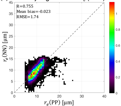
(a) Density regression of r_e (tanh)
