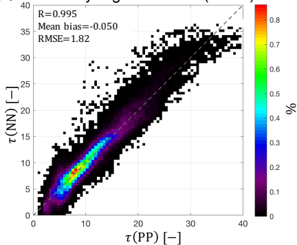
(b) Density regression of \tau (ReLU)
