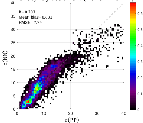
(c) Histogram of \tau (ReLU, w/ SWIR)
