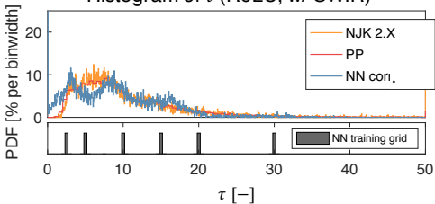
(c) Histogram of \tau (ReLU, w/ SWIR)
