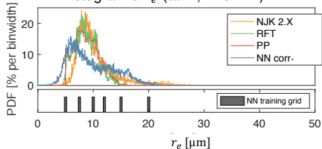
(c) Histogram of r_e (tanh, w/ SWIR)
