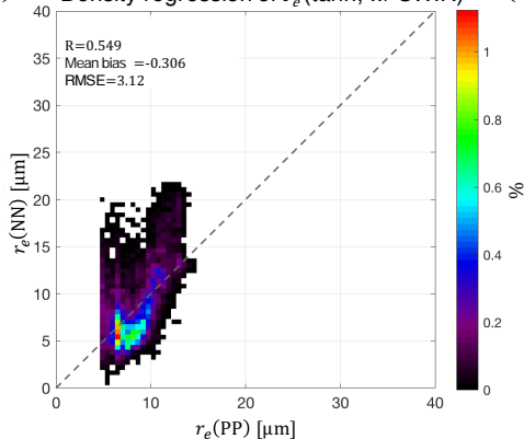
(c) Histogram of r_e (tanh, w/ SWIR)
