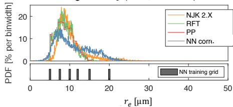
Histogram of r_e (tanh, w/ SWIR)
