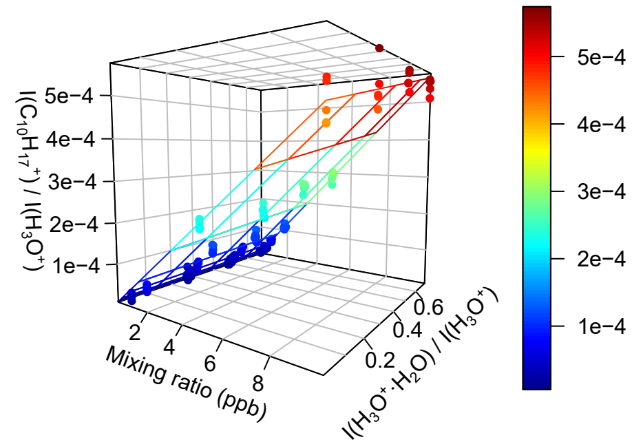
19 u / 137 u / \alpha -pinene
