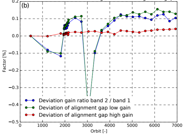
Before correction: deviation of gain ratio and alignment gaps
