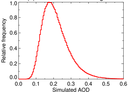
(a) Simulated AOD histogram
