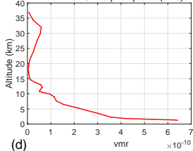
TROPOMI a priori profile (TM5)
