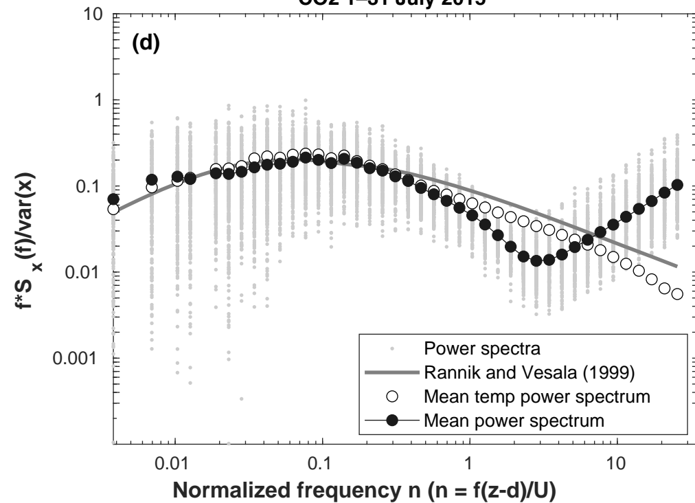
CO2 1–31 July 2015
