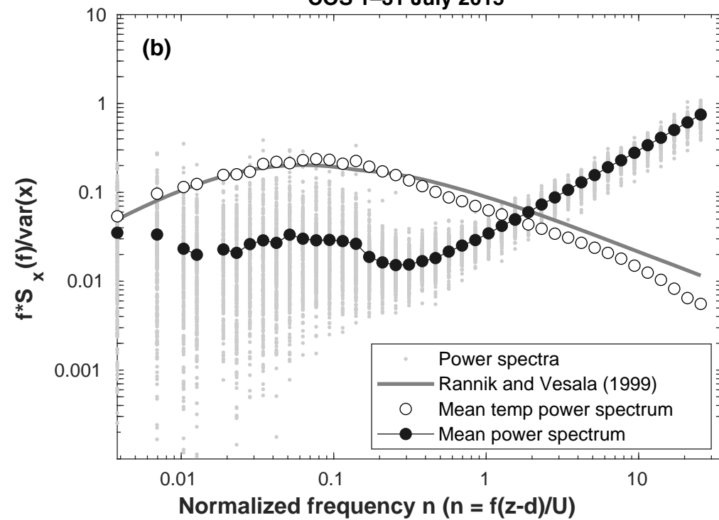
COS 1–31 July 2015
