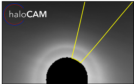
(a) Radiance, HR=1.03
