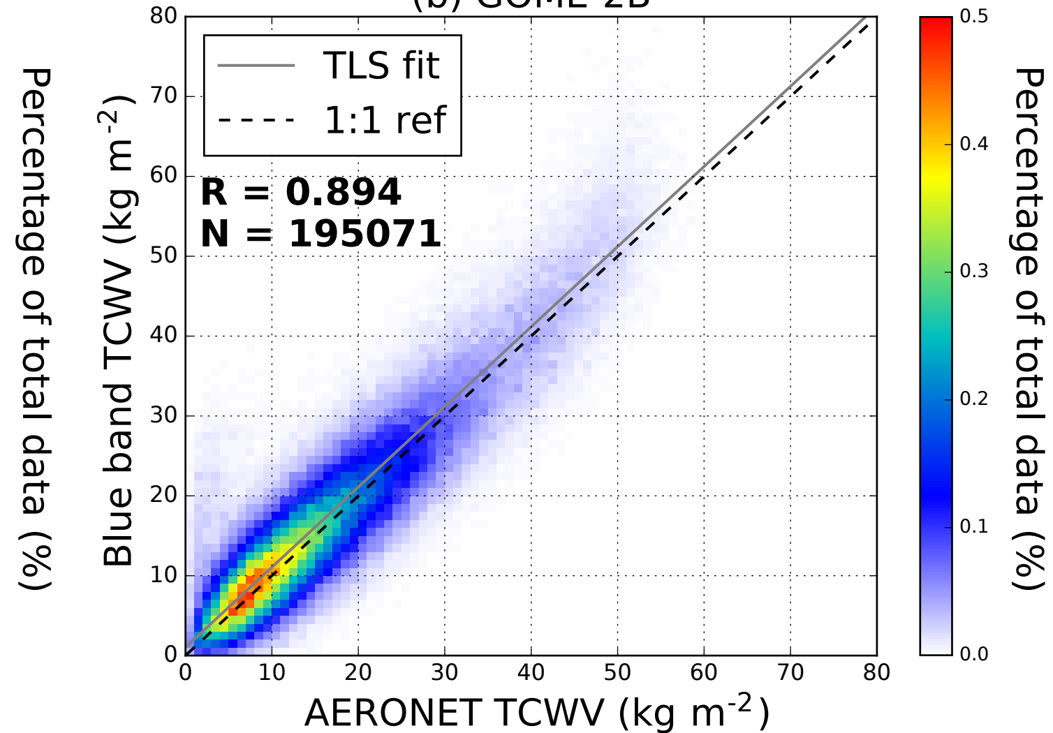
(b) GOME-2B
